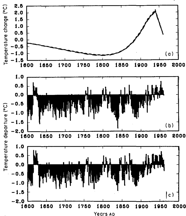
Fig. 6. (a) GTH for western Ontario; part of the GTH in Fig. 3d. (b) Single-site air temperature reconstruction from tree rings at Marquette (46°33'N, 87°24'W). (c) Single-site air temperature reconstruction from tree rings at Alpena (45°04'N, 83°26'W).
