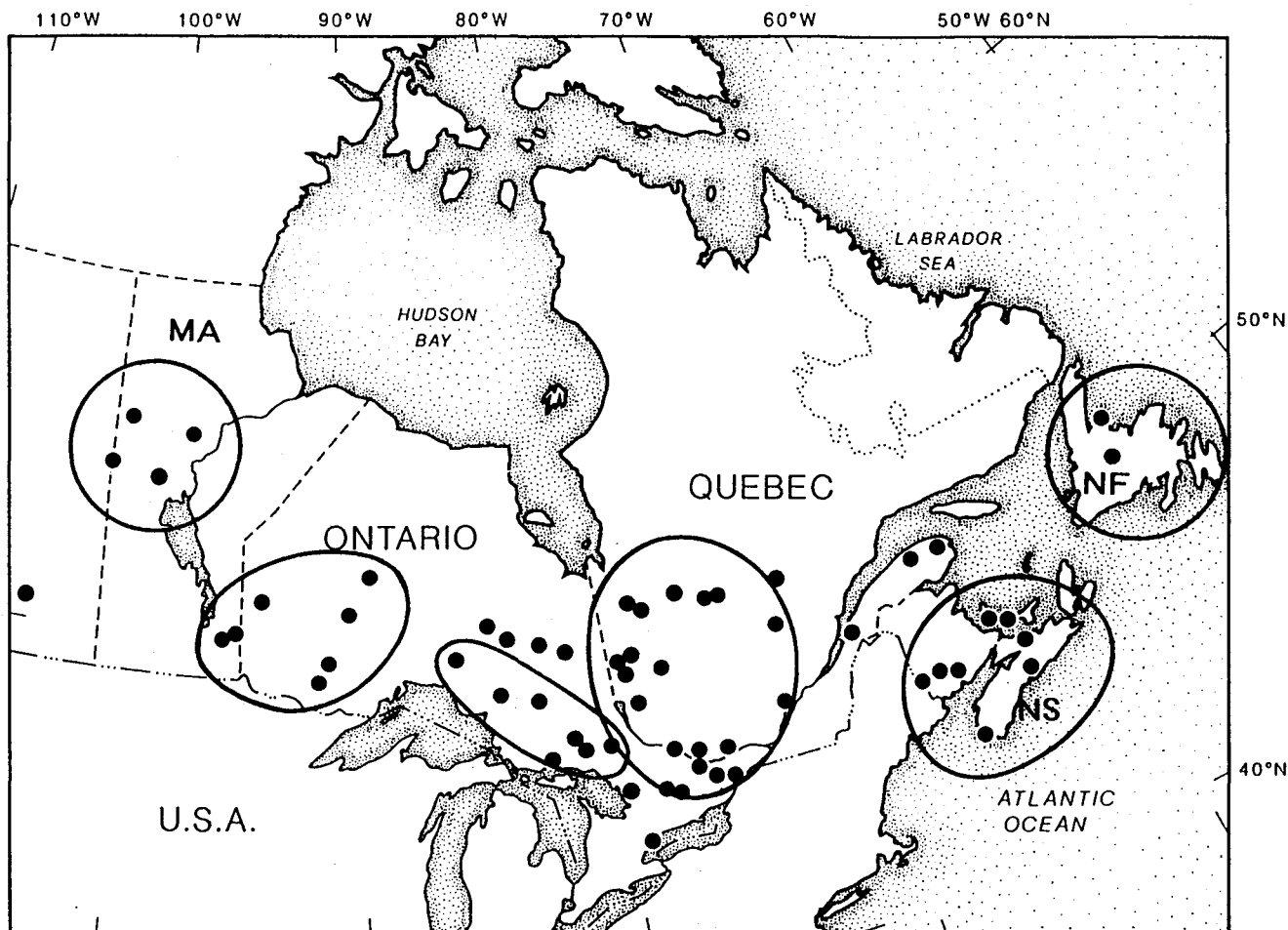
Fig. 1. Locations of sites and data used in this study. Solid lines surround the regions for which an average ground temperature history was calculated.
